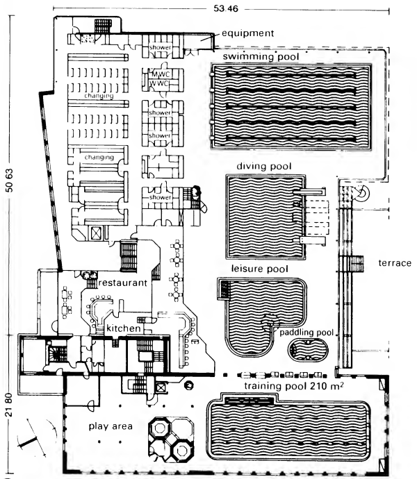
1 Trier municipal baths Architects: Muller, Karnaiz & Bock
